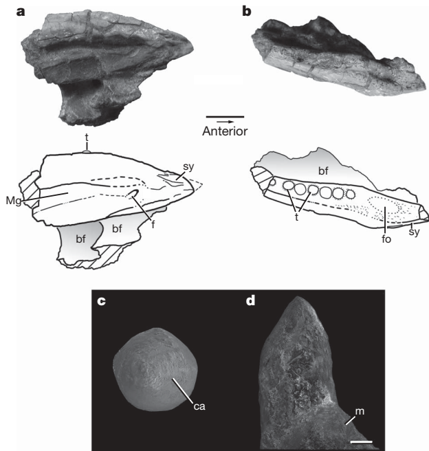
Figure 1 | New silesaurid from Tanzania, Asilisaurus kongwe (NMT RB9). a , Anterior portion of the holotypic dentary in medial view. b , Anterior portion of the holotypic dentary in occlusal view. c , d , Scanning electron micrographs of a dentary crown in occlusal ( c ) and lateral ( d ) views. Scale bars: 1 cm ( a , b ); 100 \mu m ( c , d ). bf, bone fragments; ca, carina; f, foramen; fo, fossa; m, matrix; Mg, Meckelian groove; sy, symphysis; t, tooth.
