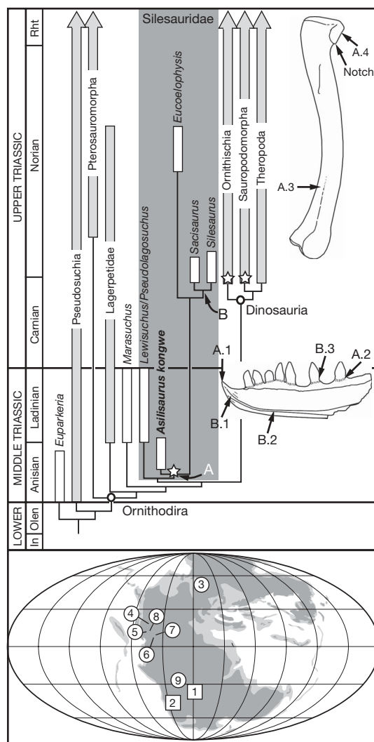
Figure 3 | Phylogenetic relationships of Asilisaurus kongwe within Archosauria and silesaurid biogeography. Strict consensus of six trees of an analysis with 33 taxa and 290 characters (Supplementary Information). Pseudosuchia, Ornithischia, Sauroptodomorpha, Theropoda, Pterosauroomorpha and Lagerpetidae have been collapsed for clarity. Stars indicate lineages with herbivorous or omnivorous diets. The length of the white bars indicates stratigraphic imprecision. Important synapomorphies for Asilisaurus plus Silesaurus illustrated on a left femur of Silesaurus in posteromedial view (top) and a right dentary of Silesaurus in medial view (bottom): A.1, anterior portion of the dentary tapers to a point; A.2, teeth fused to the bone of attachment; A.3, division of the distal condyles of the femur divided for more than one-quarter length of the element; A.4, flat articular facet of the femur. Important synapomorphies for Sacisaurus plus Silesaurus (B): B.1, Meckelian groove extends through dentary symphysis; B.2, Meckelian groove restricted to the ventral margin of dentary; B.3, teeth with constricted roots. In, Induan; Olen, Olenekian; Rht, Rhaetian. Middle Triassic (squares): 1, Asilisaurus ; 2, Lewisuchus/Pseudolagosuchus . Late Triassic taxa (circles): 3, Silesaurus ; 4, Eagle Basin specimens; 5, Petrified Forest N.P. taxon; 6, Otis Chalk taxon; 7, Technosaurus ; 8, Eucoelophysis ; 9, Sacisaurus . Palaeogeographic globe after http://jan.ucc.nau.edu/~rcb7/globaltext2.html . See Supplementary Information for further discussion of occurrences.
